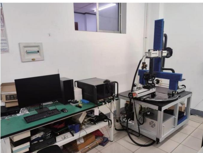
260GHz~400GHz THz topological test system
