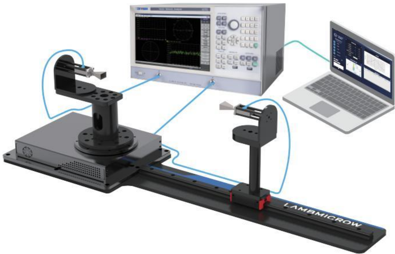
Desktop Version Teaching Solution Antenna Measurement Kit intergrating with a VNA, a set of antennas and RF cables, rotators and testing software.
