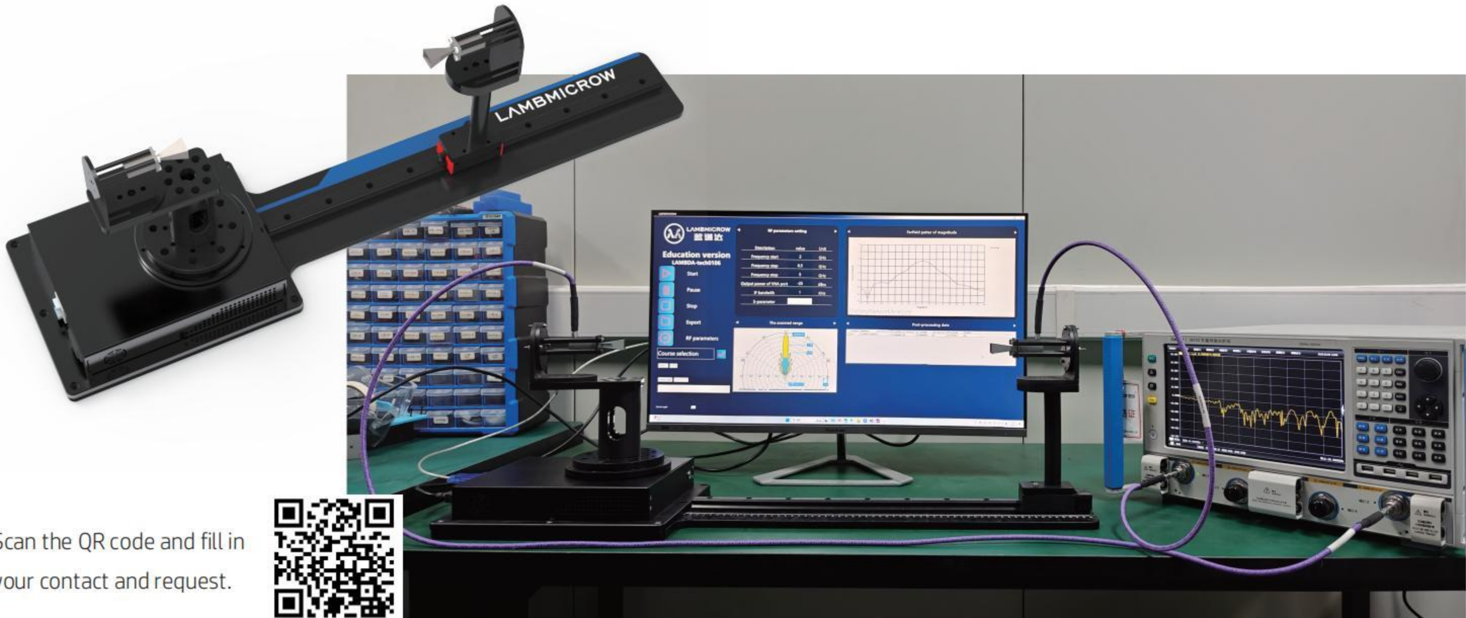
Desktop Version Teaching Solution Antenna Measurement Kit intergrating with a VNA, a set of antennas and RF cables, rotators and testing software.
