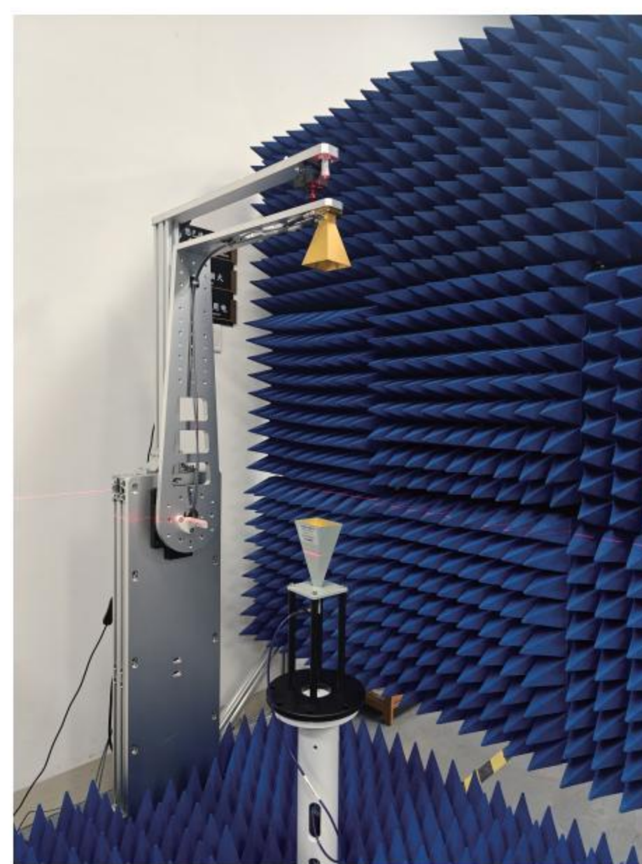
Multi-probe Test System
