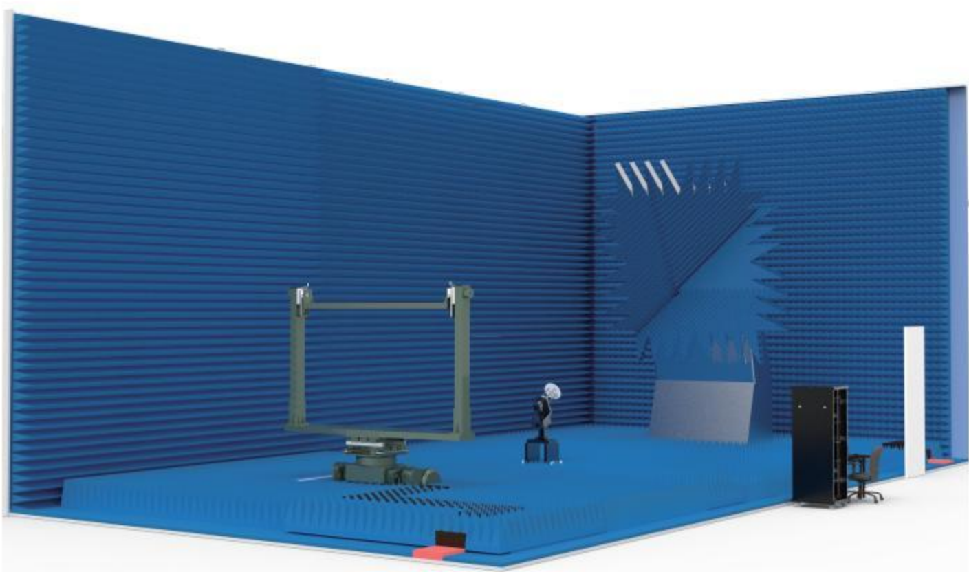
Serrated Edge Reflectors
