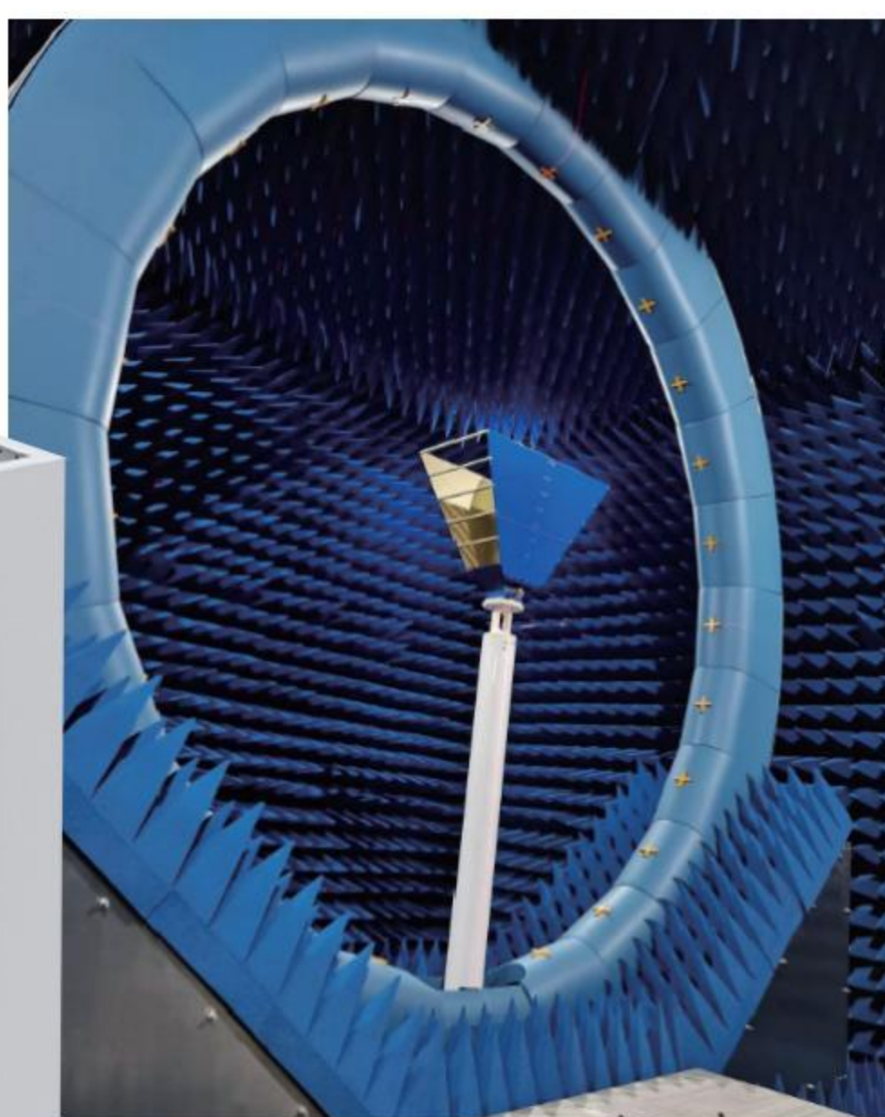
Dual-probe Test System
